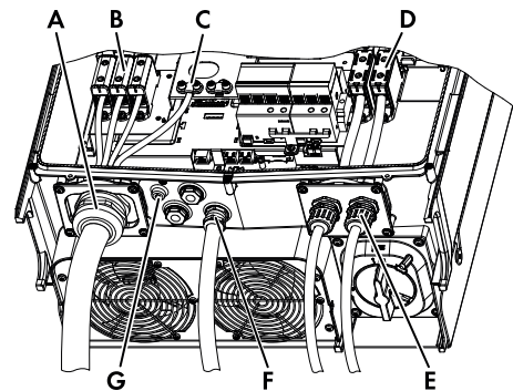
Figure 5.2 Overview of inverter with torque indications
