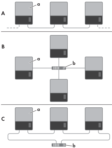
Figure 5.5 Network topology
