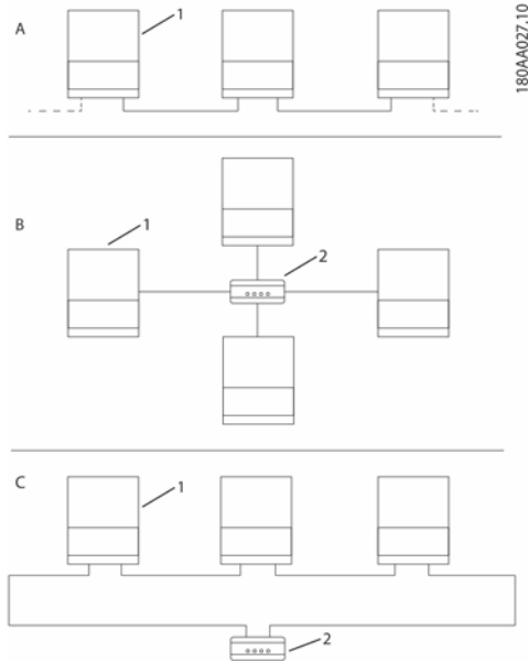
Figure 5.5 Network topology
